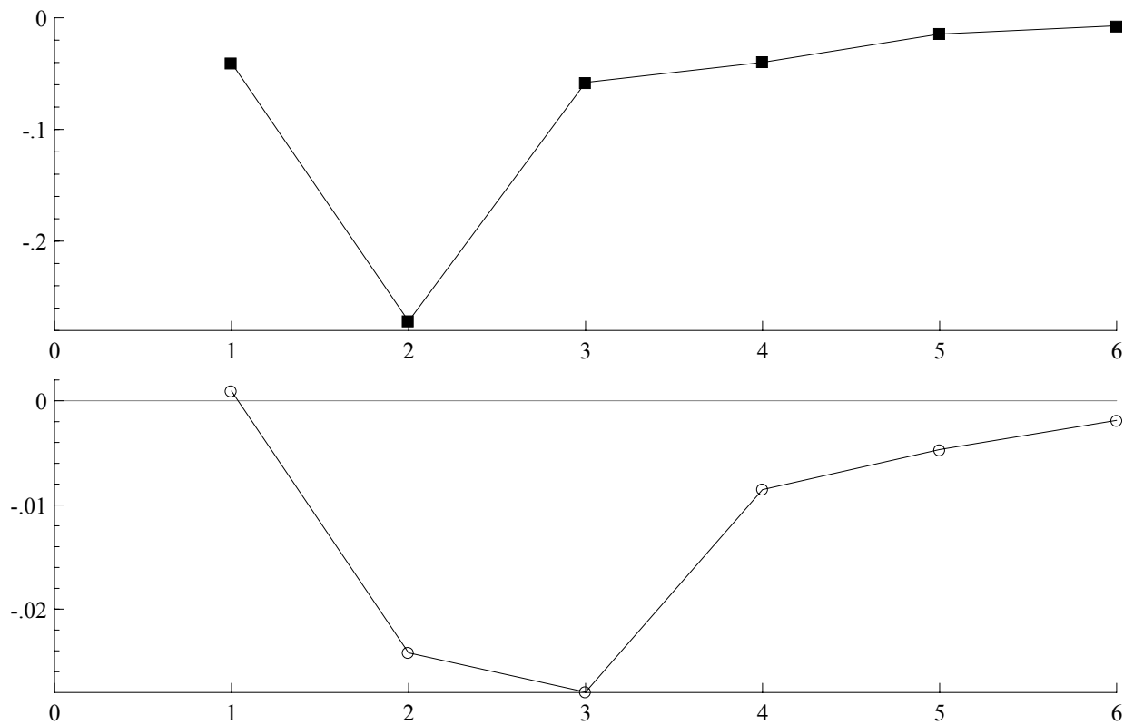
Figure 5: Response of \ln(p_{mt}/p_{nt}) to a unit increase in \ln(z_{mt}) (■) and \ln(f_{mt}) (○), European sample
